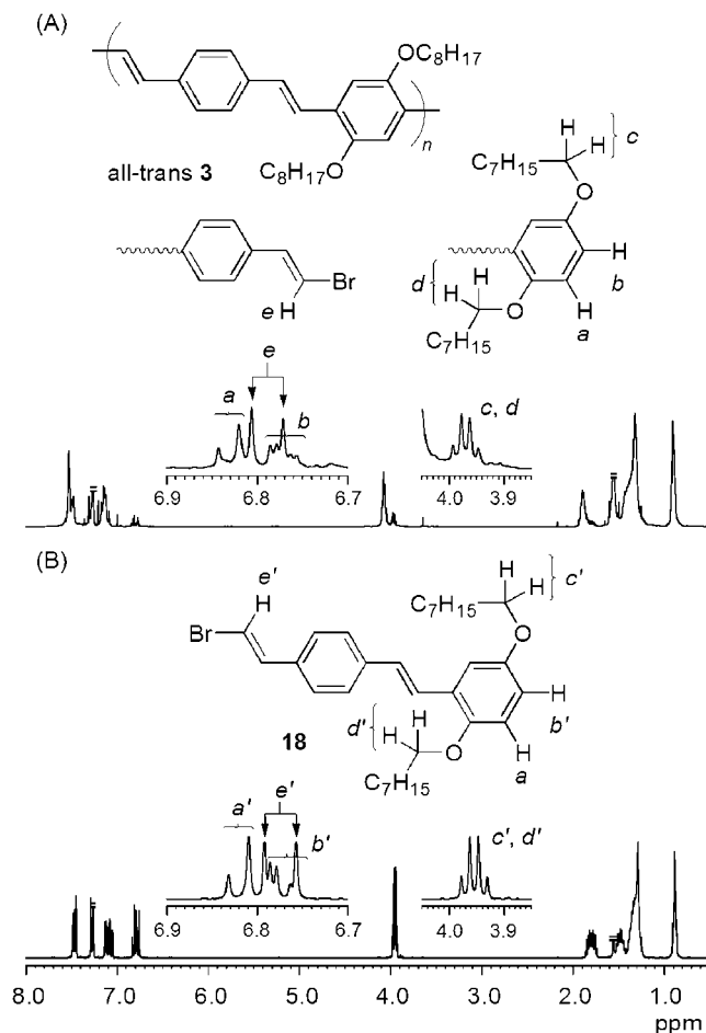
Figure 1. 1 H NMR spectra of (A) all-trans 3 (Run 2 in Table 2) and (B) 4-(2-bromoethenyl)stilbene ( 18 ) in CDCl 3 at room temperature.
