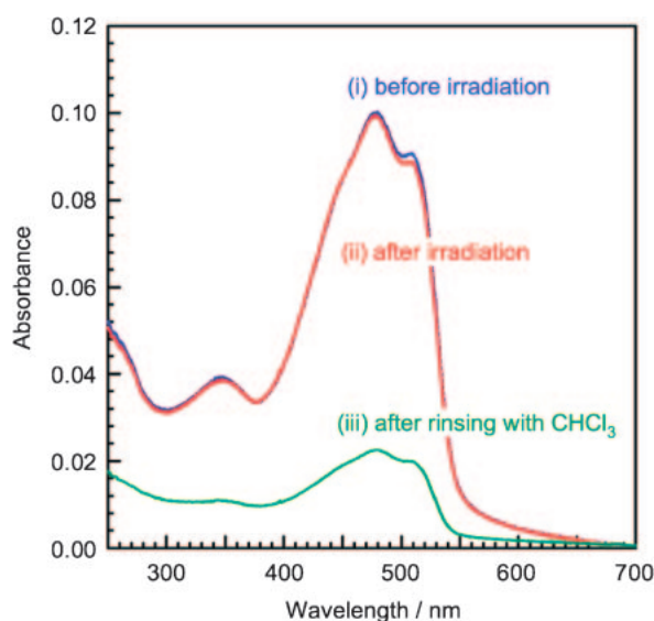
Figure 2. UV-vis absorption spectra of all-trans 3 (M n = 7500) in thin film, before and after UV-irradiation (i and ii), and after rinsing twice with CHCl 3 (iii).
